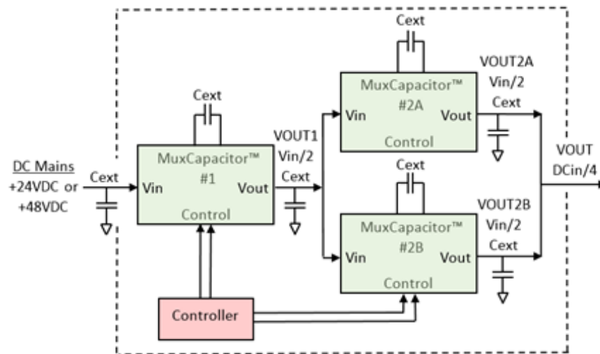
Figure 1: MxC 291 Single 12V Output EVB Block Diagram
