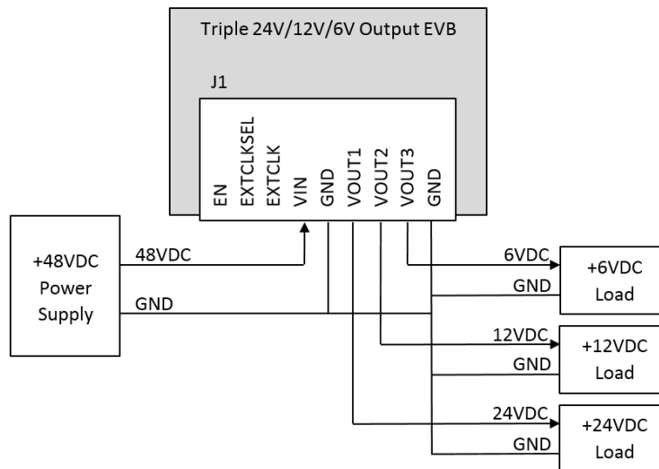
Figure 7: MxC 290 Triple Output EVB Standalone Wiring Diagram
