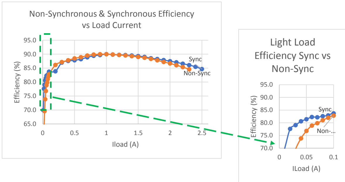
Figure 15: MxC 292 w/Synchronous Buck 5V Output EVB Efficiency Curve
