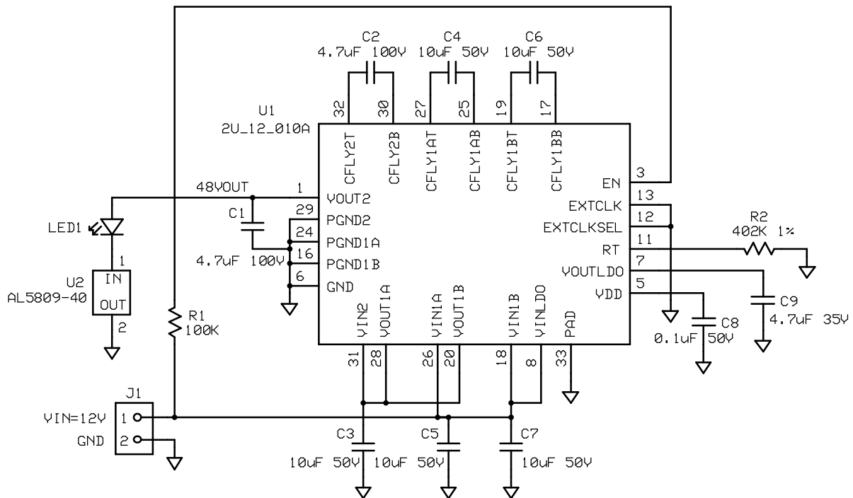
Figure 22: MxC 284 4x Voltage Boost + LED EVB Schematic
