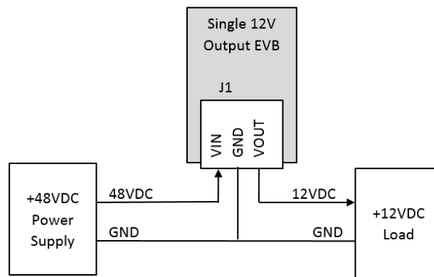
Figure 2: MxC 291 Single 12V Output EVB Standalone Wiring Diagram
